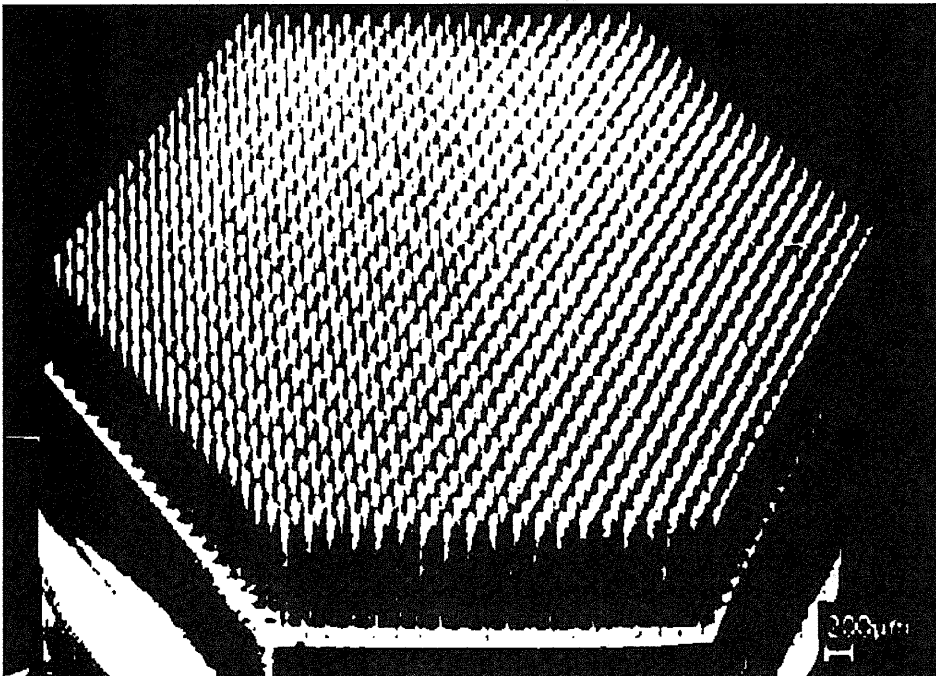
Figure 21. Scanning Electron Micrograph of a 1141 Electrode Array Made to Be Inserted Into the Surface of the Human Brain (University of Utah)
